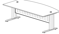
D SHAPE TABLE JD 1890 1800W x 900/750D x 750H JD 1875 1800W x 750/600D x 750H JD 1575 1500W x 750/600D x 750H
