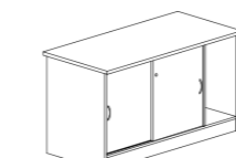
SIDE CABINET (L) EGS 1200 1200W x 500D x 750H
