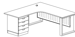
L SHAPE TABLE C/W FIXED 4D (L) SL-D 1818 1800W x 1800D x 750H SL-D 1518 1500W x 1800D x 750H SL-D 1515 1500W x 1500D x 750H SL-D 1215 1200W x 1500D x 750H
