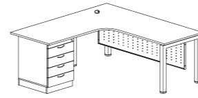
L SHAPE TABLE C/W FIXED 4D (L) UL-D 1818 1800W x 1800D x 750H UL-D 1518 1500W x 1800D x 750H UL-D 1515 1500W x 1500D x 750H UL-D 1215 1200W x 1500D x 750H
