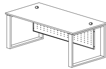
RECTANGULAR TABLE SR 1890 1800W x 900D x 750H SR 1875 1800W x 750D x 750H SR 1575 1500W x 750D x 750H SR 1275 1200W x 750D x 750H
