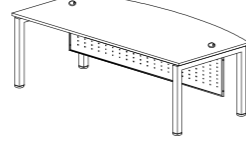
D SHAPE TABLE UD 1890 1800W x 900/750D x 750H UD 1875 1800W x 750/600D x 750H UD 1575 1500W x 750/600D x 750H
