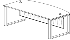
D SHAPE TABLE SD 1890 1800W x 900/750D x 750H SD 1875 1800W x 750/600D x 750H SD 1575 1500W x 750/600D x 750H
