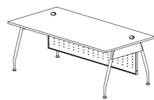
RECTANGULAR TABLE AR 1890 1800W x 900D x 750H AR 1875 1800W x 750D x 750H AR 1575 1500W x 750D x 750H AR 1275 1200W x 750D x 750H
