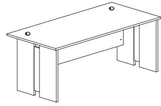
WRITING TABLE FM - 187 1800W x 700D x 750H FM - 157 1500W x 700D x 750H FM - 127 1200W x 700D x 750H
