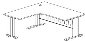
L SHAPE TABLE (L) JL 1818 1800W x 1800D x 750H JL 1518 1500W x 1800D x 750H JL 1515 1500W x 1500D x 750H JL 1215 1200W x 1500D x 750H
