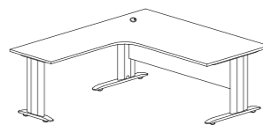
L SHAPE TABLE C/W WOODEN MODESTY & 1 LEG (L) MT 1518R 1500W x 1800D x 750H
