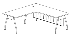
L SHAPE TABLE (L) AL 1818 1800W x 1800D x 750H AL 1518 1500W x 1800D x 750H AL 1515 1500W x 1500D x 750H AL 1215 1200W x 1500D x 750H
