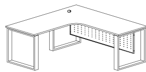
L SHAPE TABLE (L) SL 1818 1800W x 1800D x 750H SL 1518 1500W x 1800D x 750H SL 1515 1500W x 1500D x 750H SL 1215 1200W x 1500D x 750H
