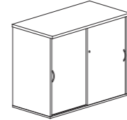
SLIDING DOOR CABINET FM - SD 800W x 410D x 820H
