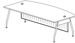
D SHAPE TABLE AD 1890 1800W x 900/750D x 750H AD 1875 1800W x 750/600D x 750H AD 1575 1500W x 750/600D x 750H
