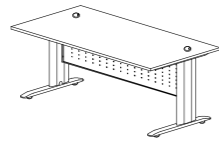
RECTANGULAR TABLE JR 1890 1800W x 900D x 750H JR 1875 1800W x 750D x 750H JR 1575 1500W x 750D x 750H JR 1275 1200W x 750D x 750H
