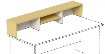
COUNTERISER FM - C18 1800W x 300D x 300H FM - C15 1500W x 300D x 300H FM - C12 1200W x 300D x 300H
