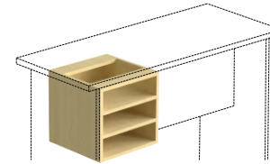
RETURN RACK FO - RS 302W x 345D x 335H
