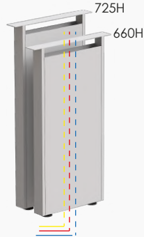
WIRE MANAGEMENT WM 725 300W x 50D x 725H WM 660 300W x 50D x 660H
