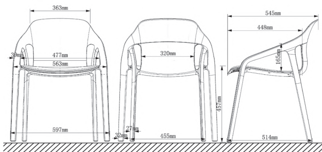
Product Size Diagram
