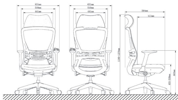
Product Size Diagram
