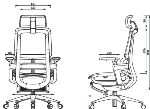
Product Size Diagram
